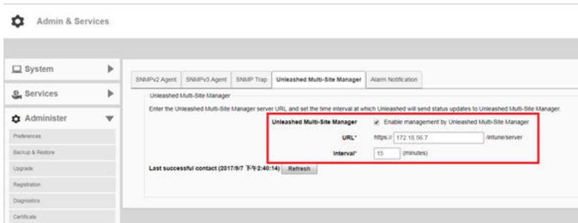
FIGURE 74 Enabling Unleashed Multi-Site Manager Management
